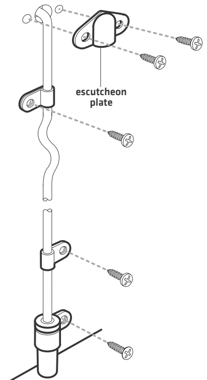
Routing the Temp Probe Cable
