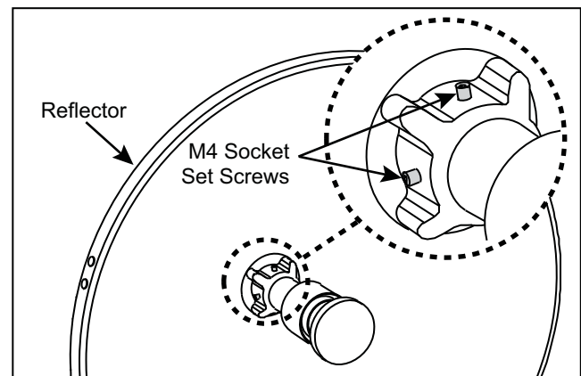
Figure 54: LNB Skew Angle Adjustment
