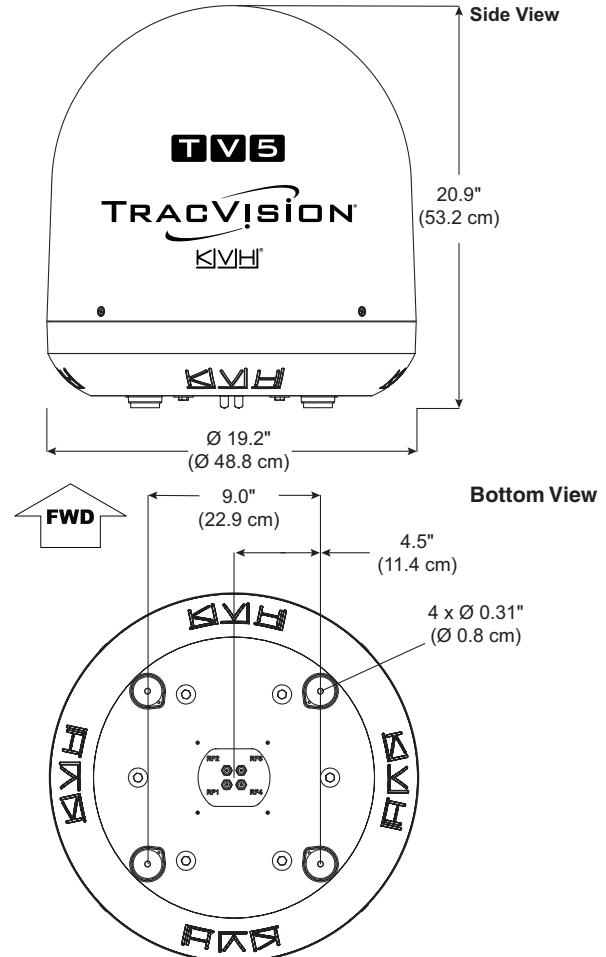
Figure 5: Antenna Dimensions
