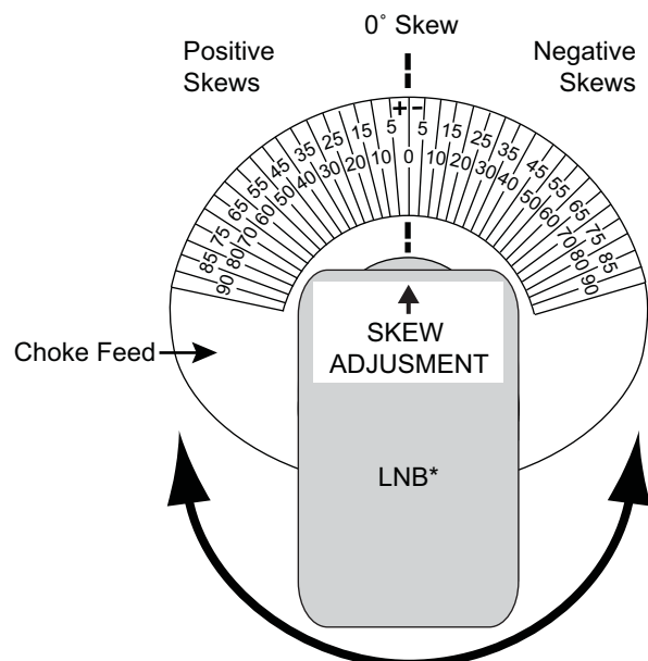
Figure 54: LNB Skew Angle Adjustment
