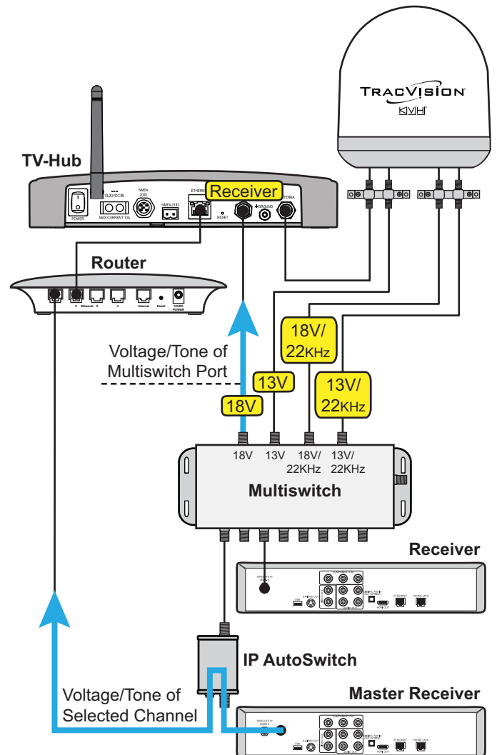
Figure 64: Linear Receivers with Multiswitch and IP AutoSwitch
