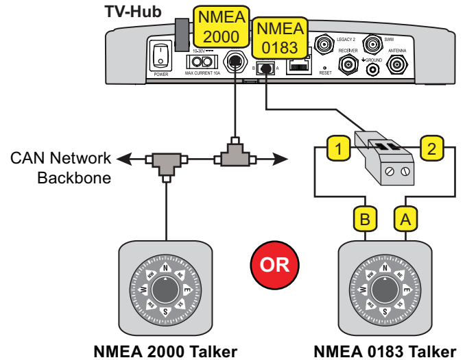
Figure 35: TV-Hub NMEA Connections
