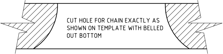
SECTION A-A OF DECK
